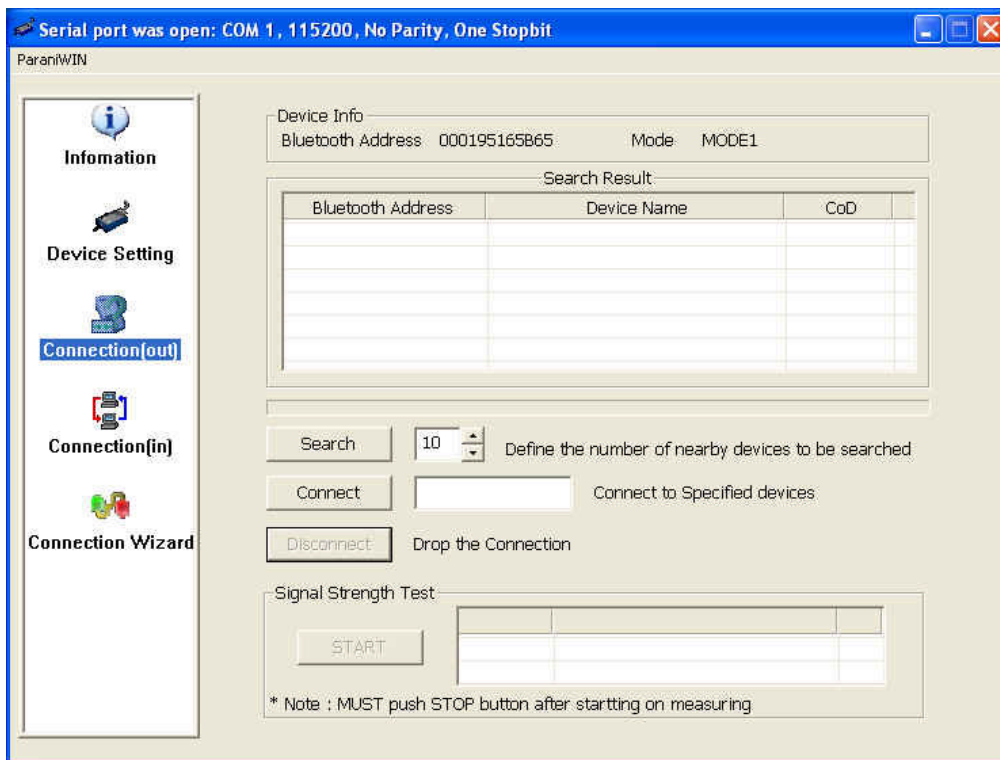
Figure 3-8 Connect(out) Window
