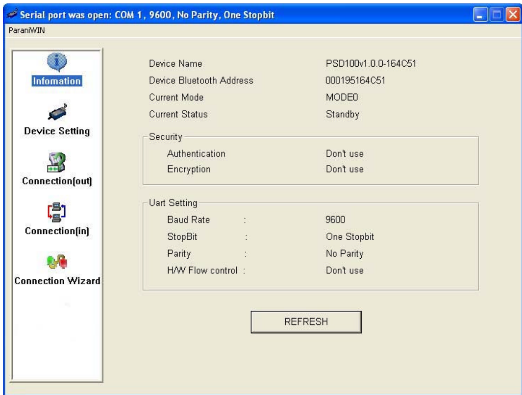
Figure 3-4 Main Window
