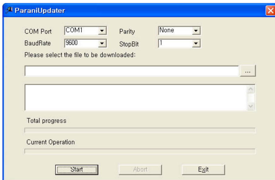
Figure 3-12 ParaniUpdater Window
